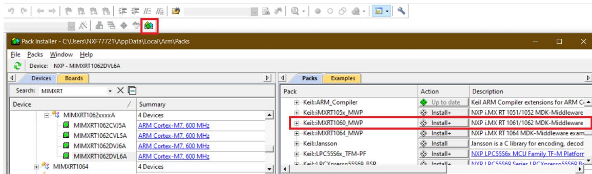
Figure 20: Install Packages using Pack Installer in Keil
